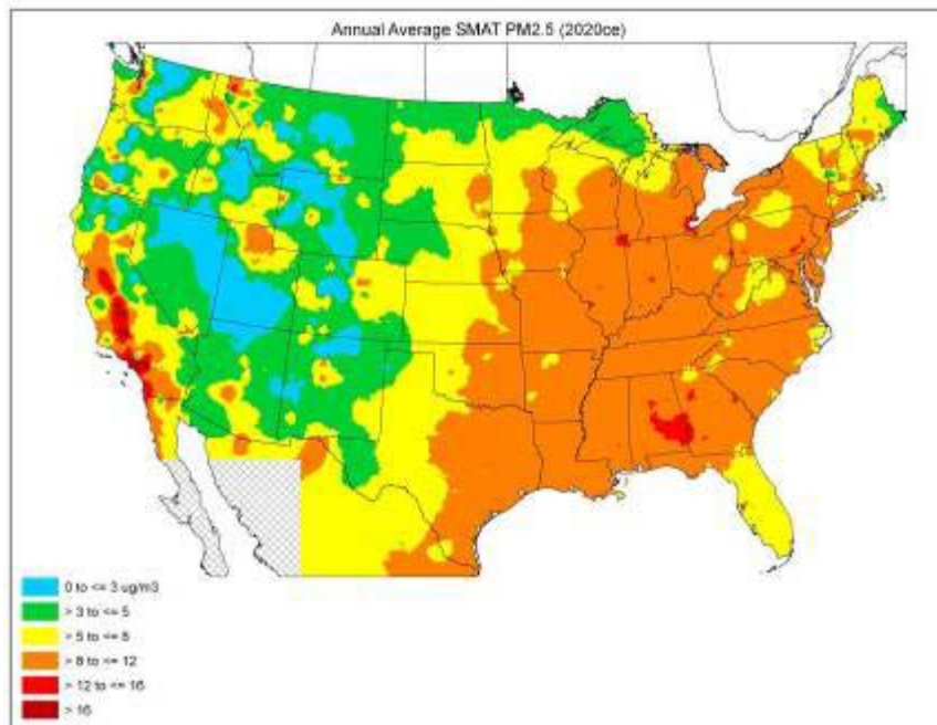
Figure 3.3-1 – PM 2.5 Annual Mean Concentration for Current Performance Scenario in the United States in 2020
