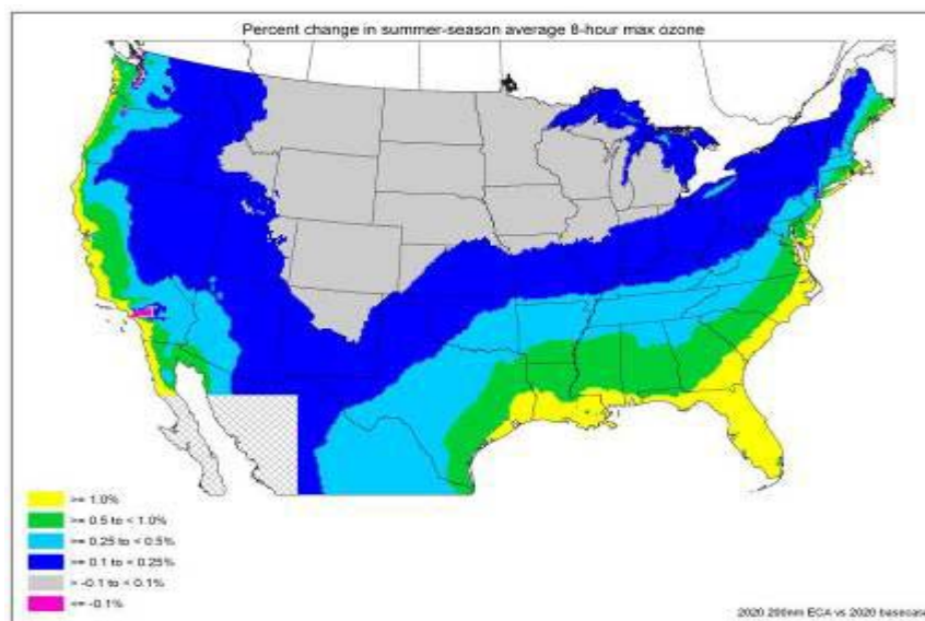
Figure 3.3-10 – Per cent Improvement in Average Daily Maximum 8-hour Ozone Concentrations in 2020 Resulting from the Application of the Proposed ECA
