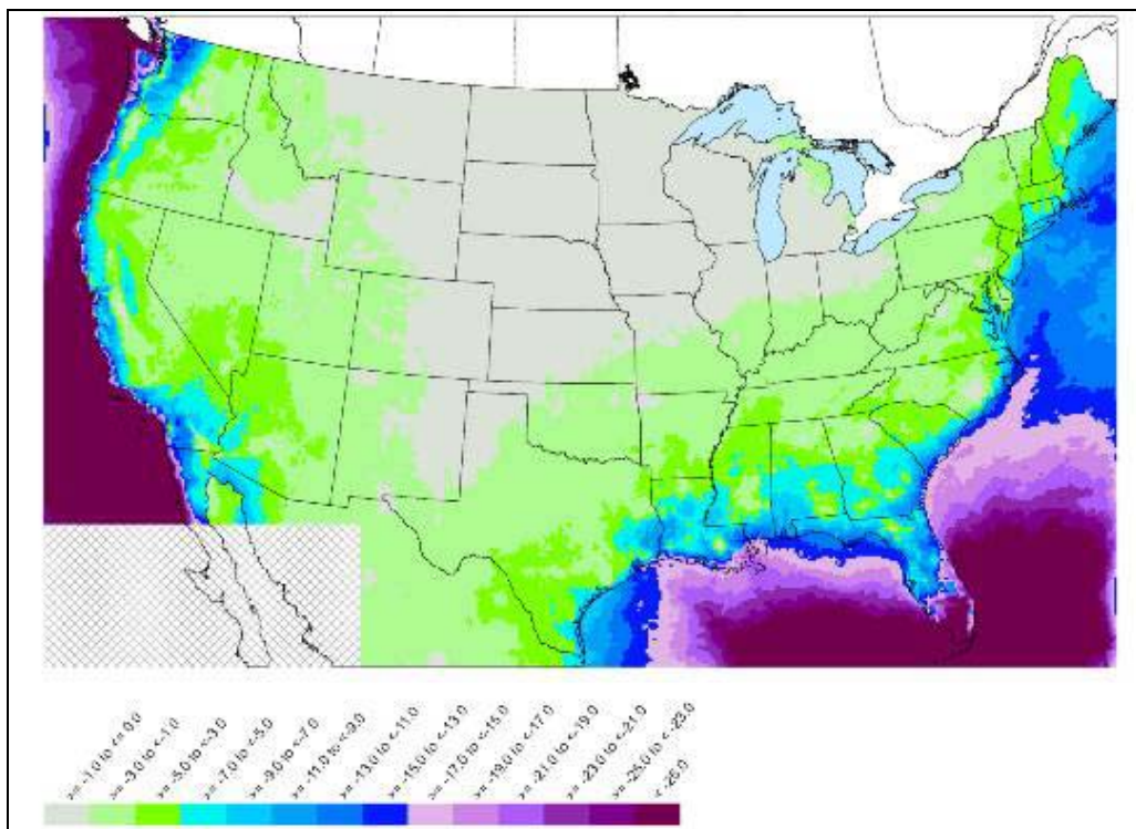
Figure 5.1 – 6 Per cent Contribution of Ships to Annual United States Total Nitrogen Deposition in 2020
