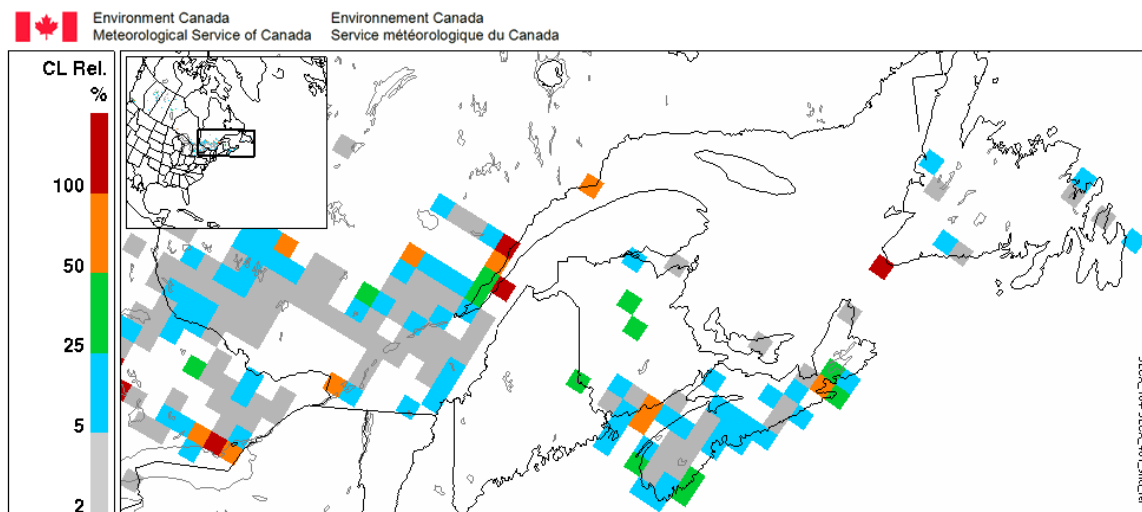
Figures 5.1-10 – Per cent Reduction in Excess Sulphur and Nitrogen in Southwestern British Columbia (top), and the Atlantic Coast (bottom), for the Proposed ECA Compared to Current Ship Emissions Performance.
