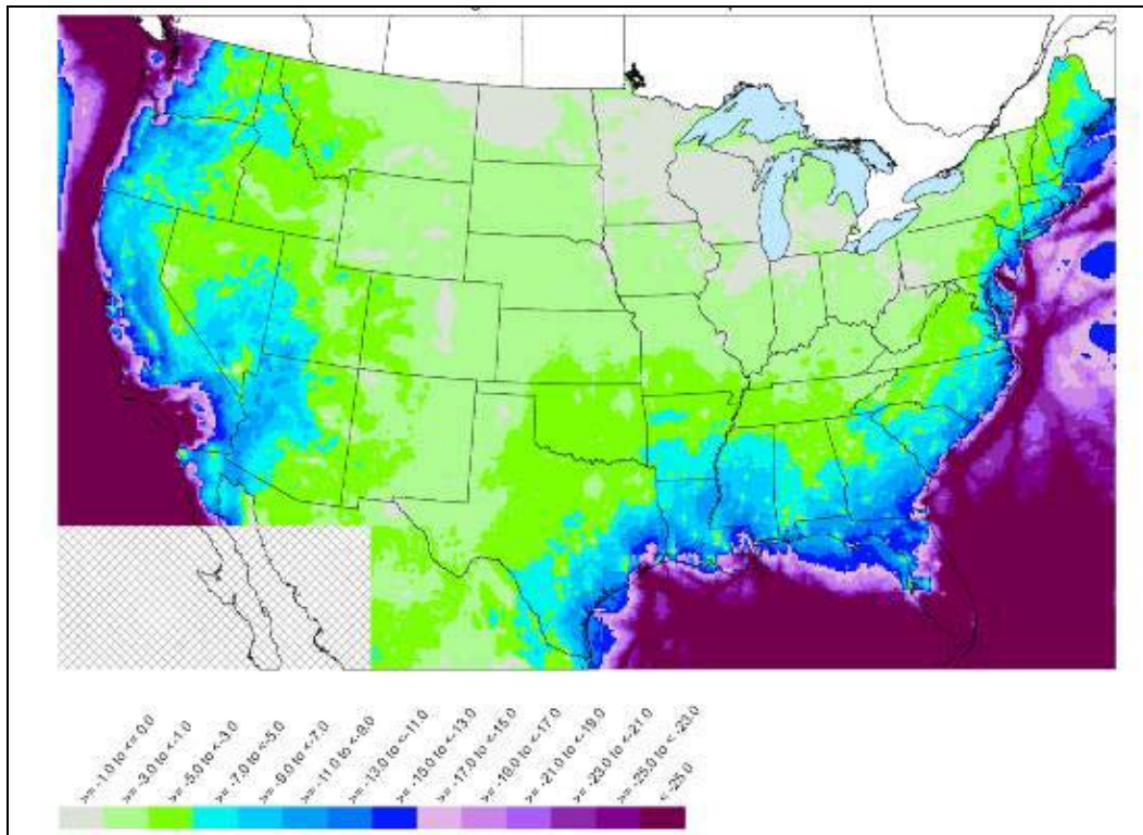
Figure 5.1 – 5 Per cent Contribution of Ships to Annual United States Total Sulphur Deposition in 2020
