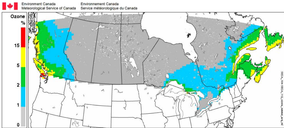
Figure 3.3-8 – Ships’ Contribution to Ozone in 2020.
