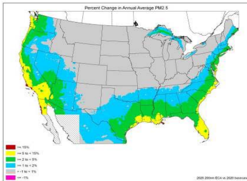
Figure 3.3-9 – Per cent Improvement in Annual Average PM_{2.5} Concentrations in 2020 Resulting from the Application of the Proposed ECA
