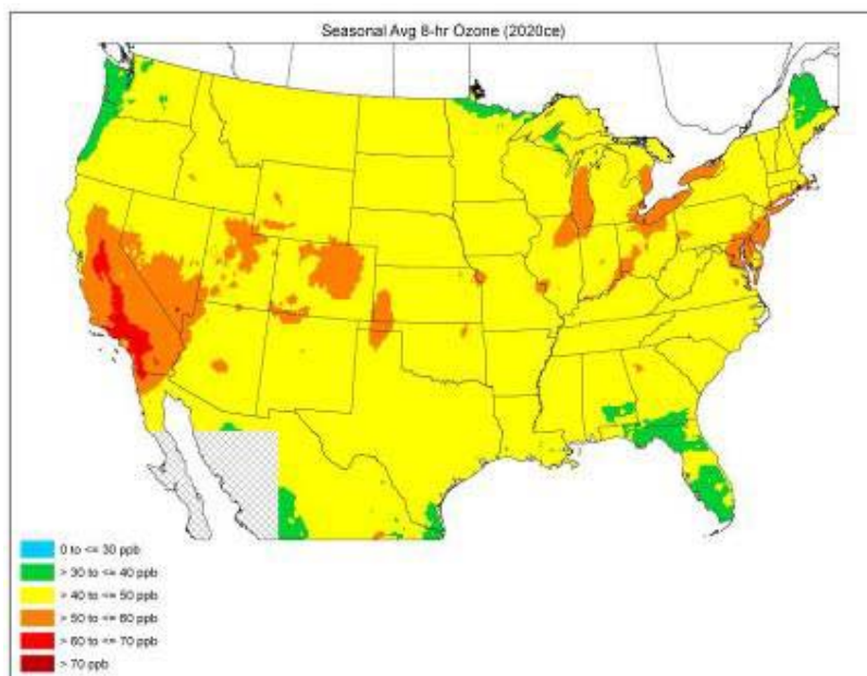
Figure 3.3-3 – Projected Seasonal Average 8-hour Maximum Ozone Levels (ppb) for Current Performance Scenario in the United States in 2020
