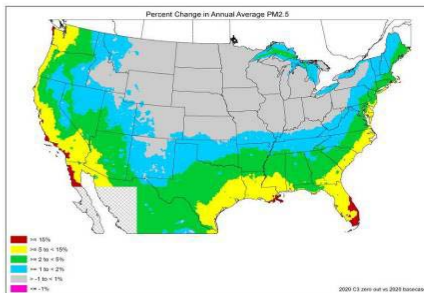
Figure 3.3-2 – Per cent Contribution of Ships to Annual Average PM 2.5 Concentrations in 2020
